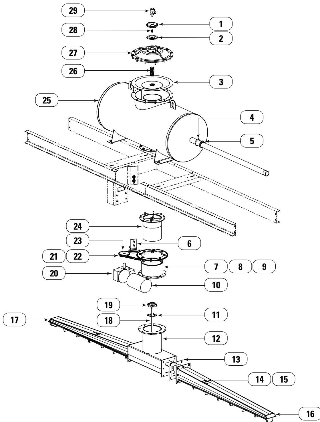
Air Tank, RFW and RFWH 232-484
