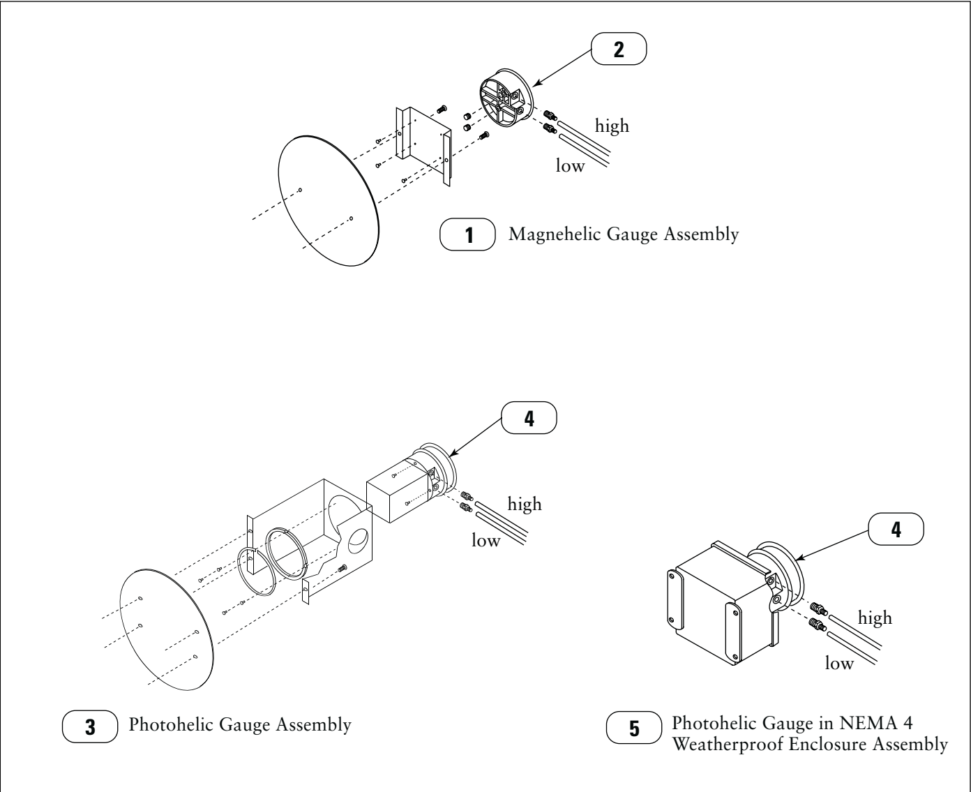
Magnehelic and Photohelic Gauge Assembly
