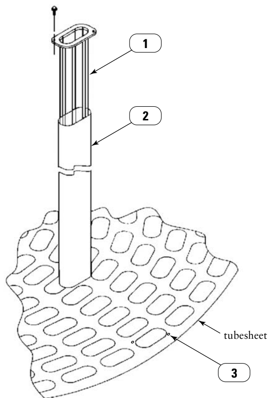
Filter and Cage, Boltsafe Hardware
