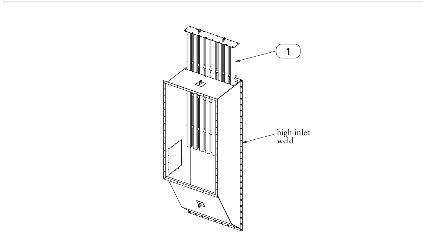
High Inlet Baffle Weld, RFWH
