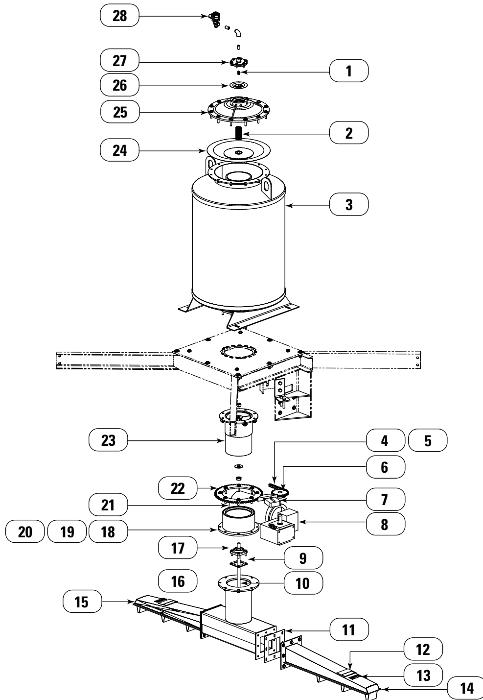
Air Tank, RFW and RFWH 124-156
