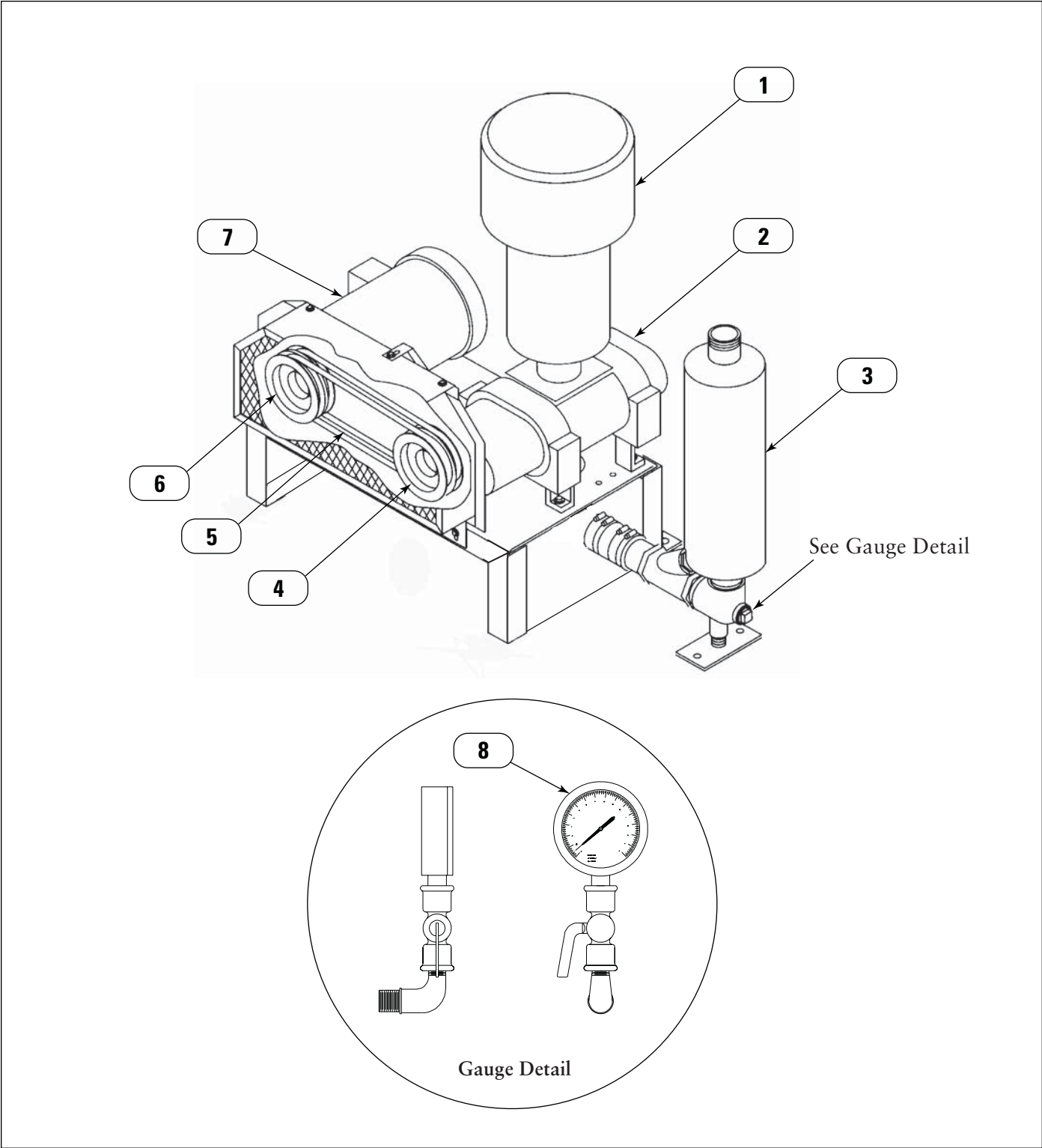
Positive-Displacement Blower
