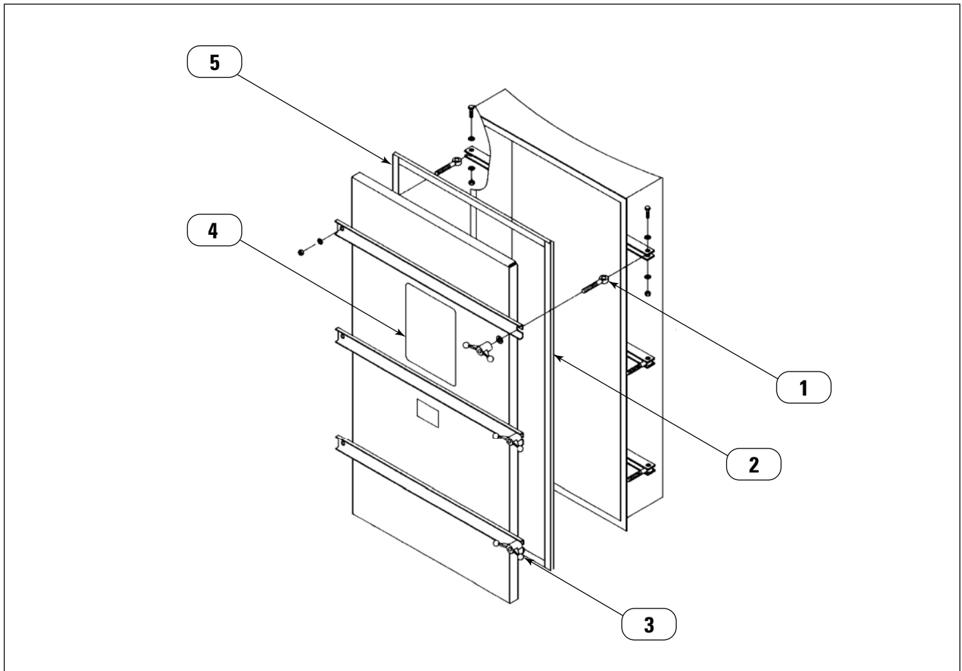
Access Panel, RFW and RFWH
