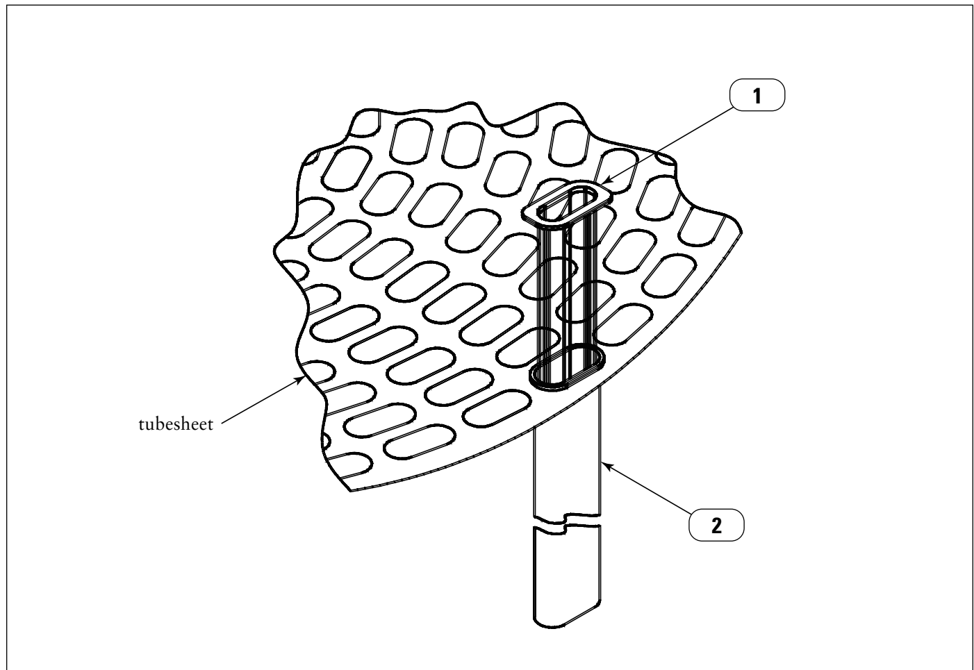
Filter and Cage, Snap-In
