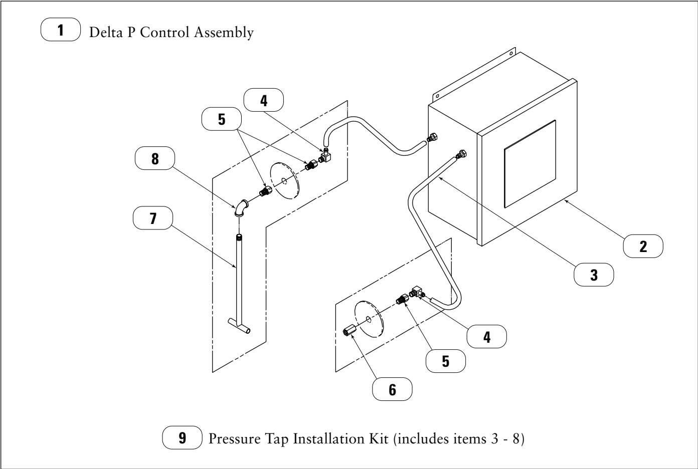
Delta P Control Assembly
