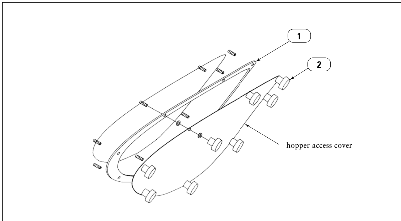
Hopper Access
