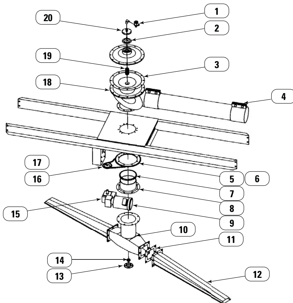
Cleaning System, RFW, RFWH, and RFT 48-72
