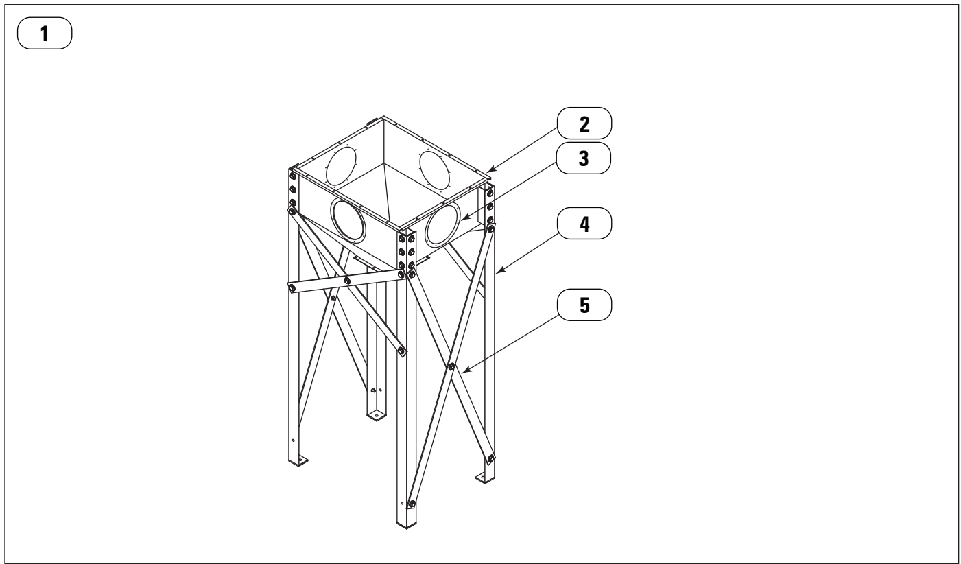
Hopper and Leg Assembly for 55-Gallon Drum
