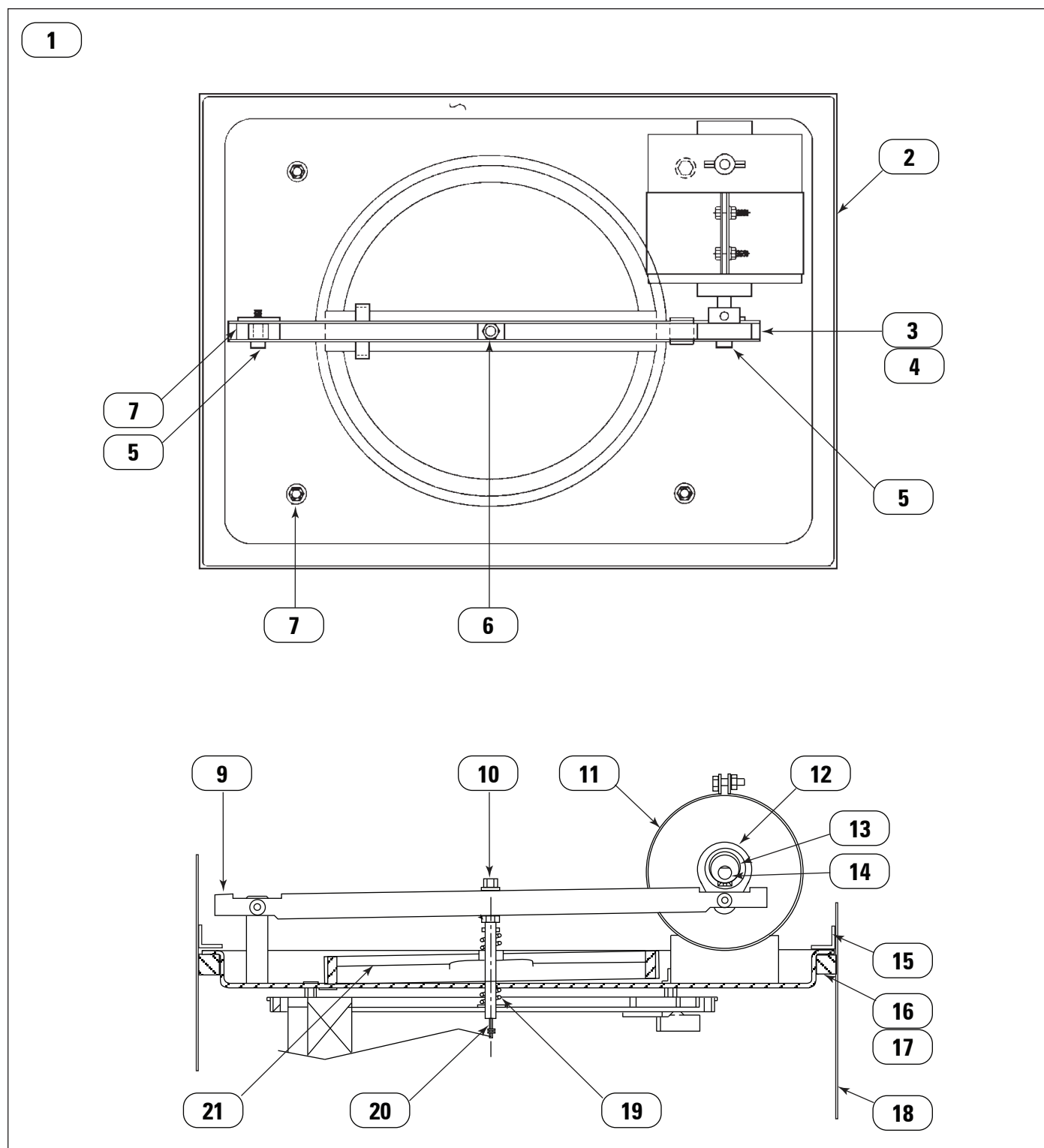
Shaker Panel Assembly, Units Built Before February 1999
