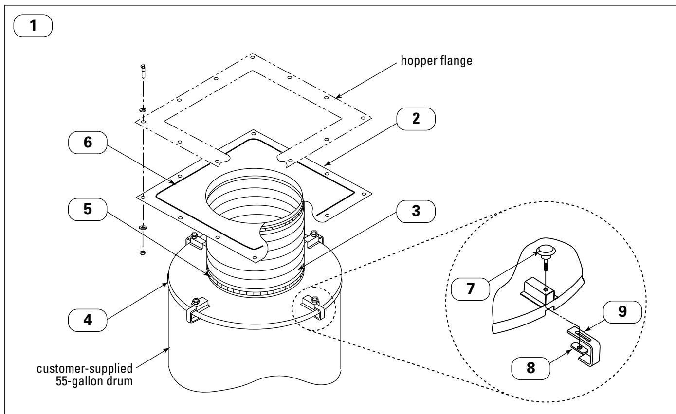
Drum Cover Assembly
