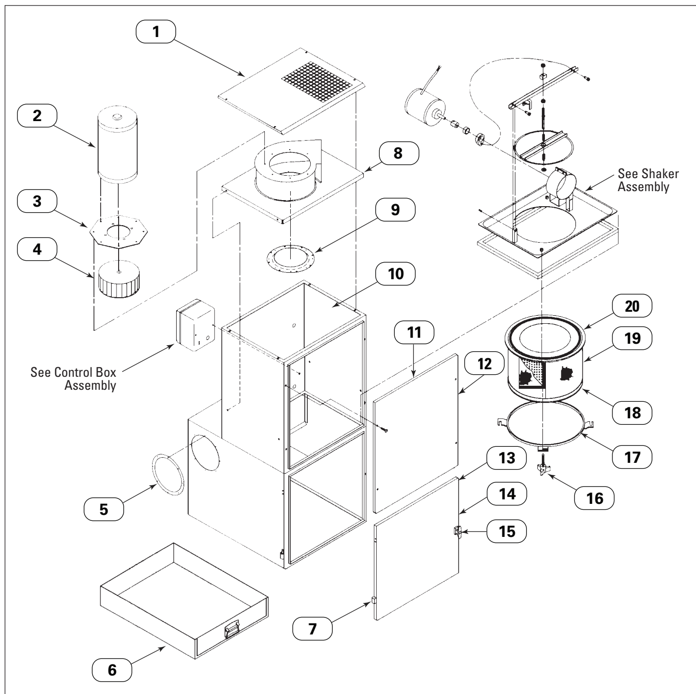
VS-550, 1200, and 1500
