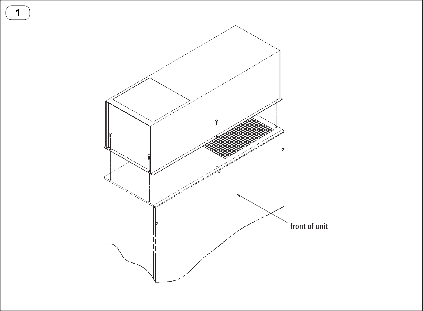
Silencer Assembly
