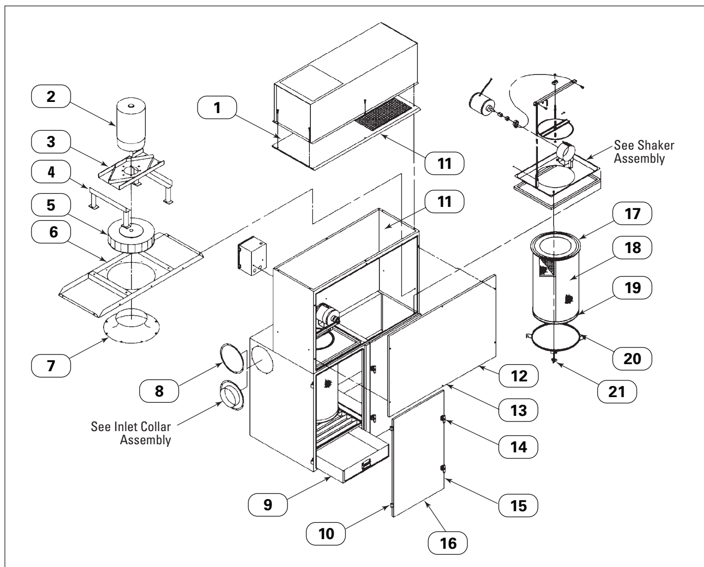
VS-2400 and 3000
