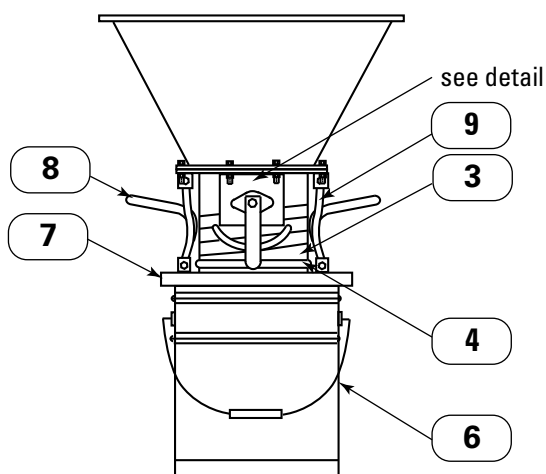
2 5-Gallon Pail Pack with Gate Valve
