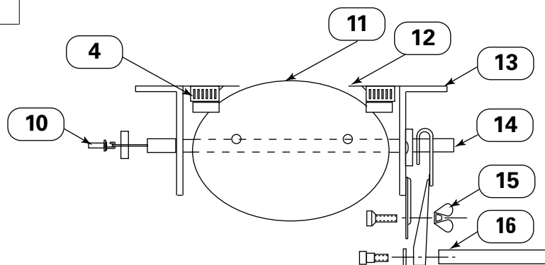
Side View Gate Valve
