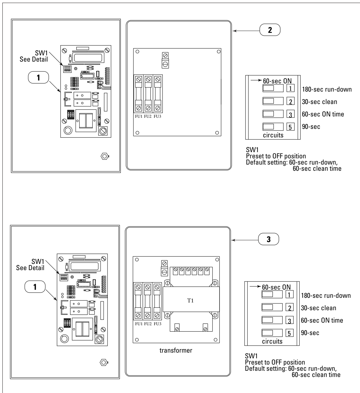
Control Box Assembly
