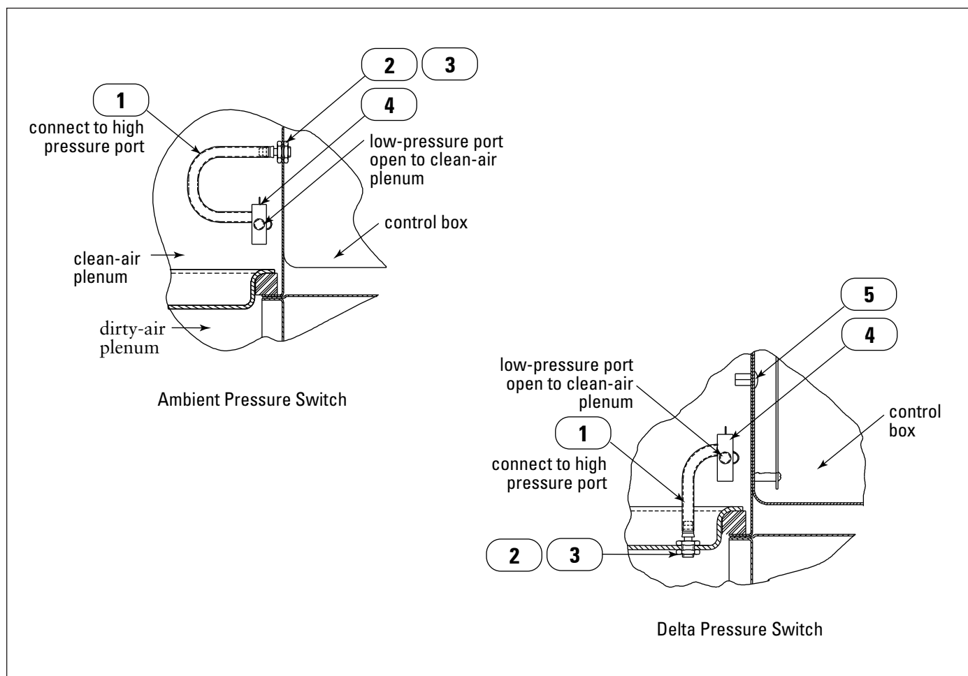
Pressure Switches
