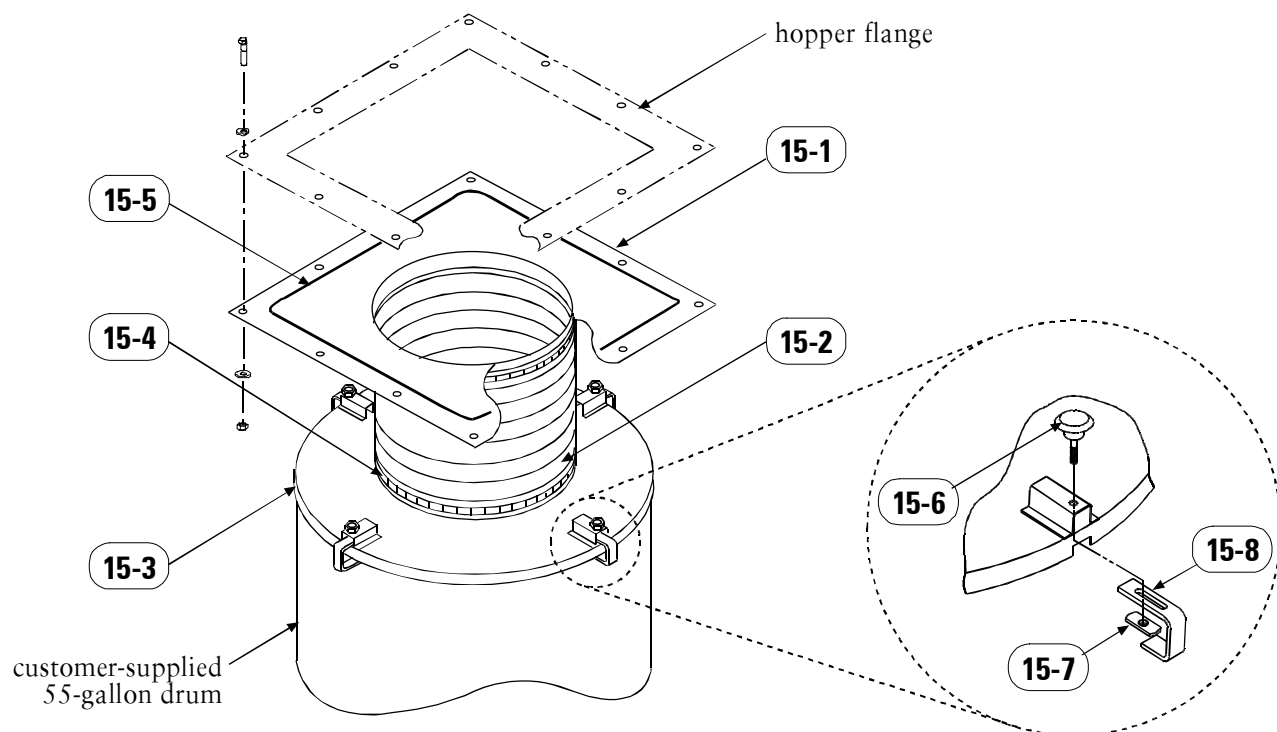
Parts Drawing 15, Drum Cover Assembly
