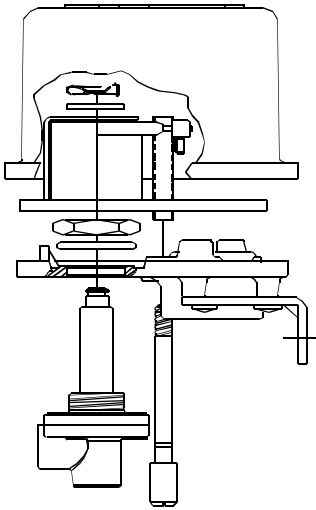
11-3 Solenoid Valve with Coil, 1/8-in NPT
