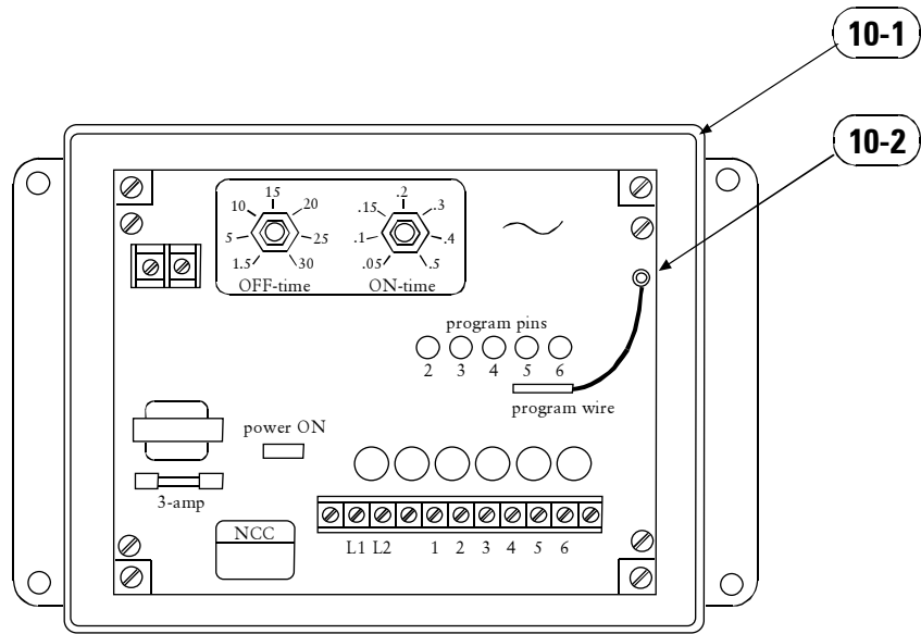
10 Control Box and Timer Assembly
