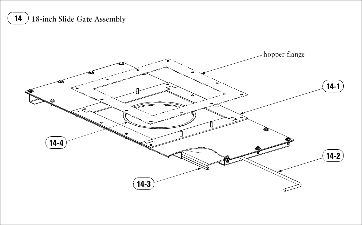
Parts Drawing 14, Slide Gate Assembly
