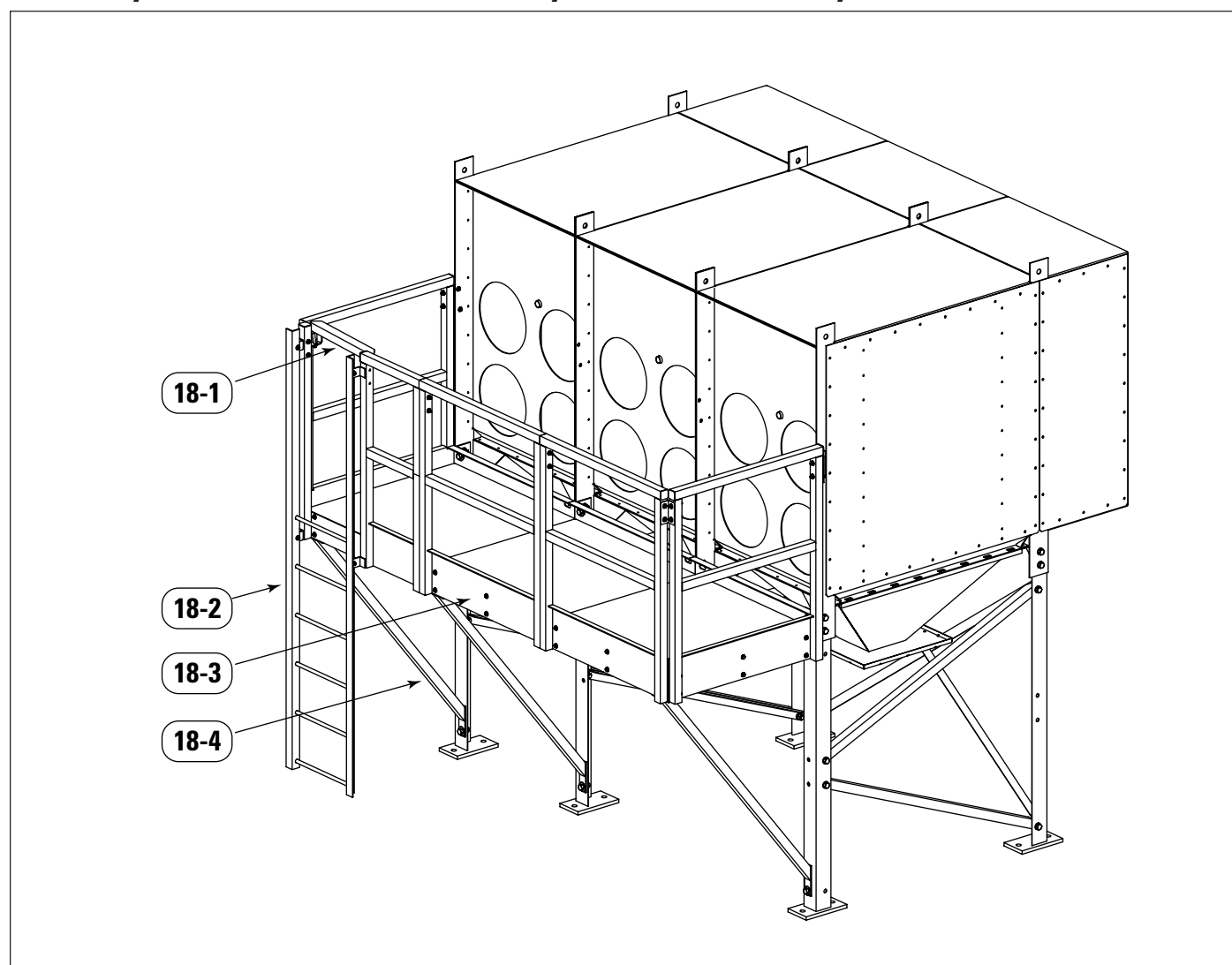
Parts Drawing 18, Stationary Ladder and Platform Assembly
