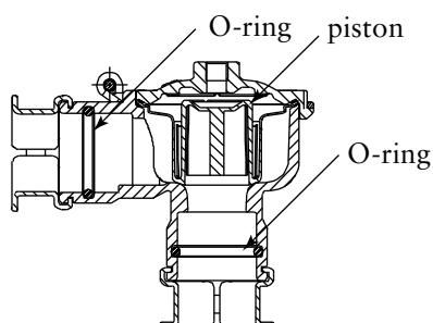
8-1 Diaphragm Valve Repair Kit, 1-in ASCO
