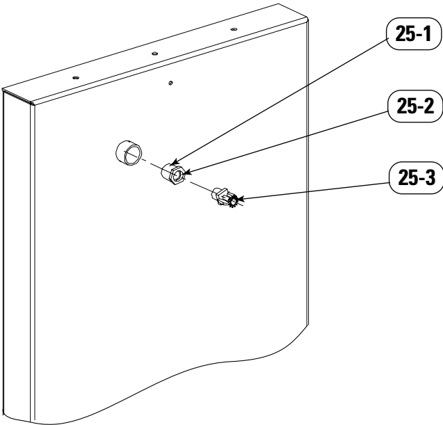
Parts Drawing 25, Sprinkler Assembly
