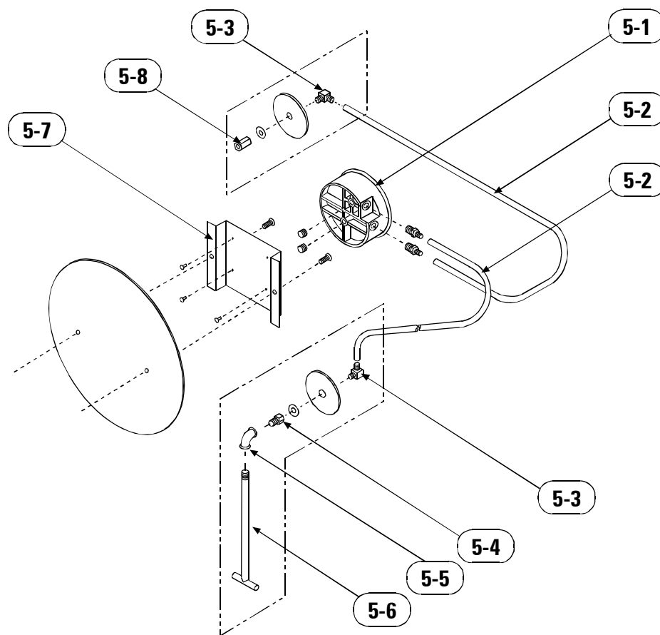
Parts Drawing 5, Magnehelic Gauge Assembly
