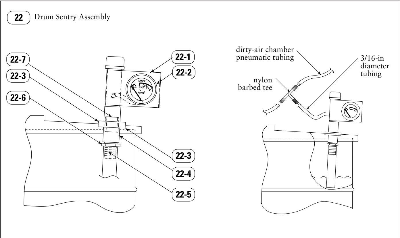
Parts Drawing 22, Drum Sentry
