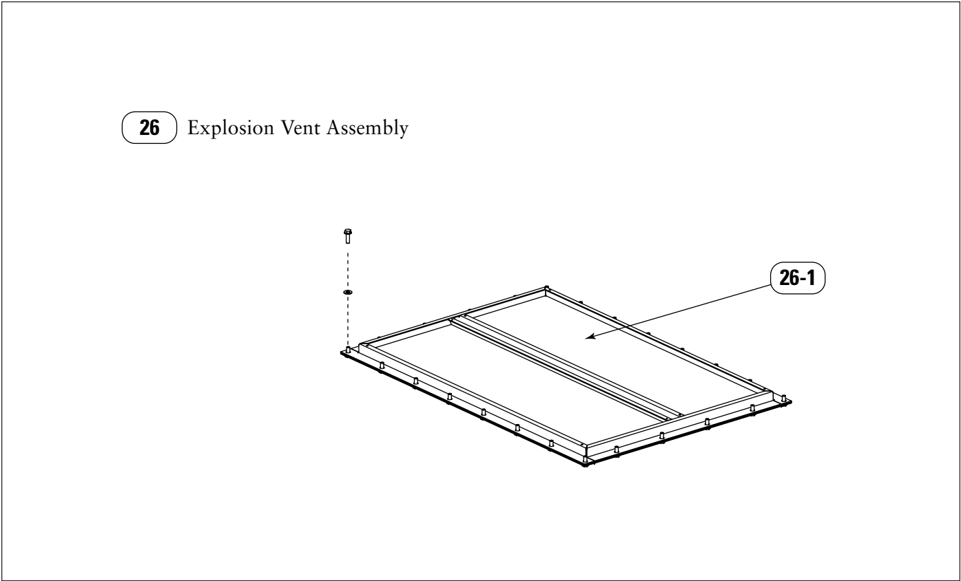
Parts Drawing 26, Explosion Relief Vent
