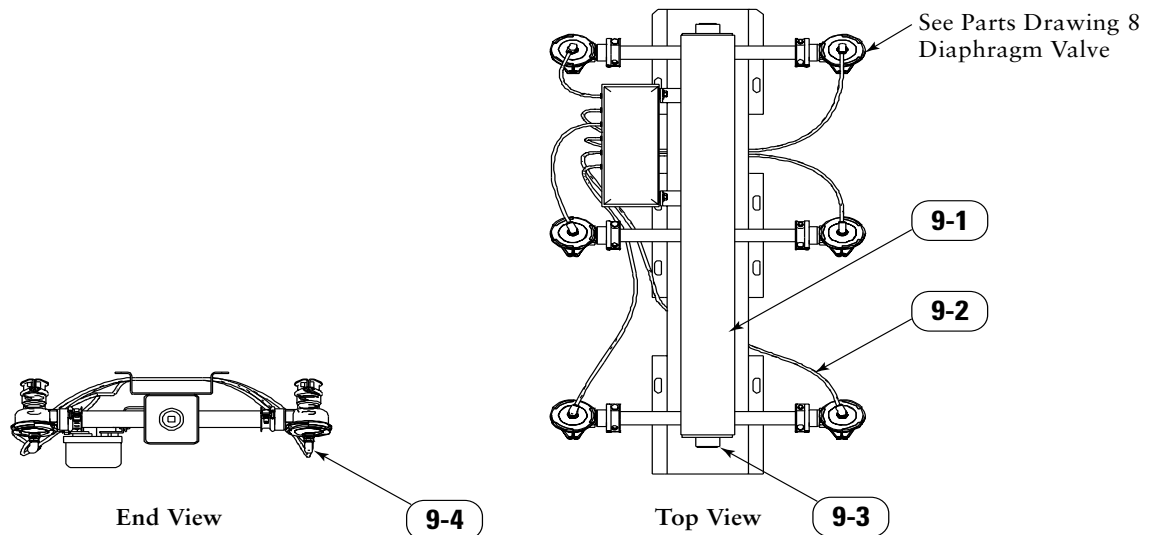
Parts Drawing 9, Manifold Assembly
