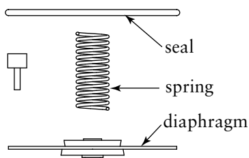
8-1 Diaphragm Valve Repair Kit, Goyen RCAC25
