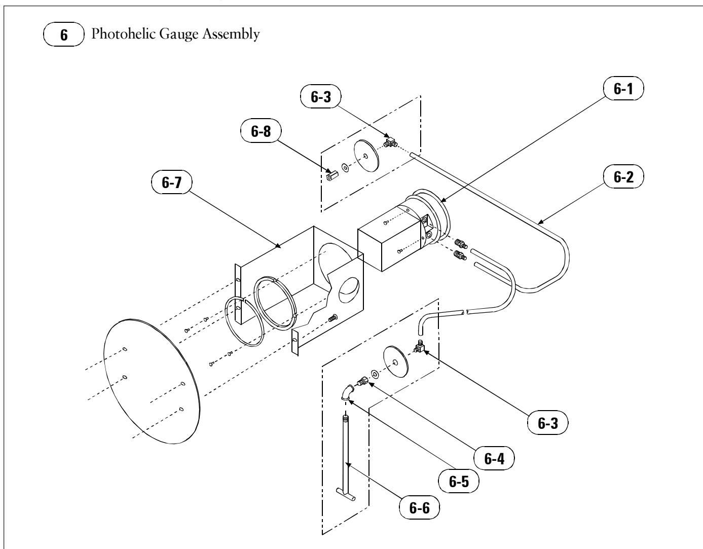
Parts Drawing 6, Photohelic Gauge Assembly
