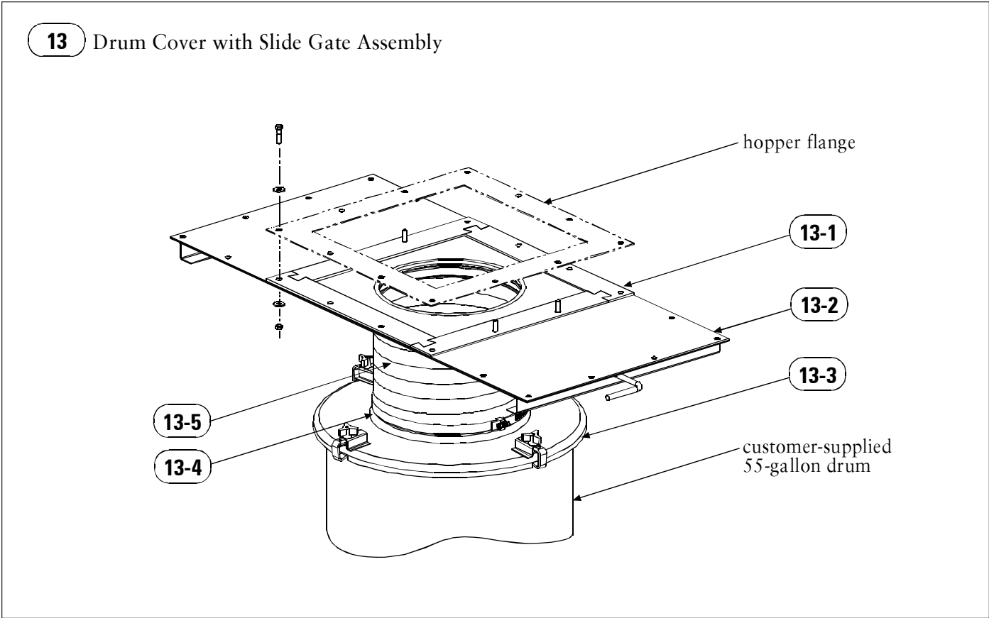
Parts Drawing 13, Drum Cover with Slide Gate Assembly
