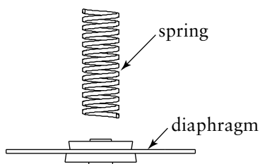
8-1 Diaphragm Valve Repair Kit, Goyen RCA25
