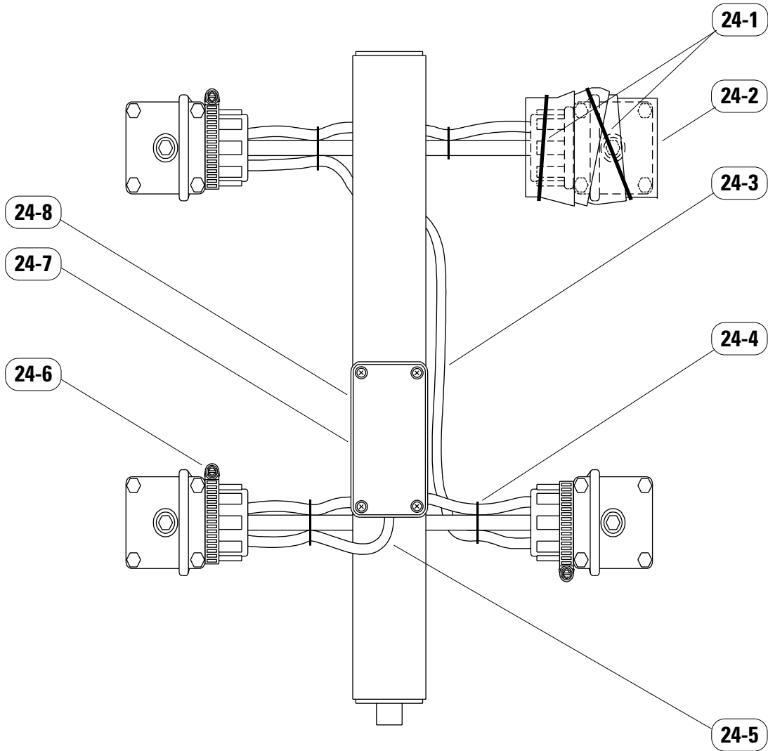
Parts Drawing 24, Heavy-Duty Cold-Climate Kit
