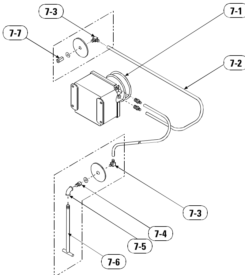
Parts Drawing 7, Photohelic Gauge in NEMA 4 Weatherproof Enclosure Assembly
