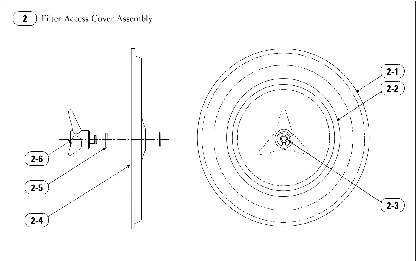
Parts Drawing 2, Filter Access Cover Assembly
