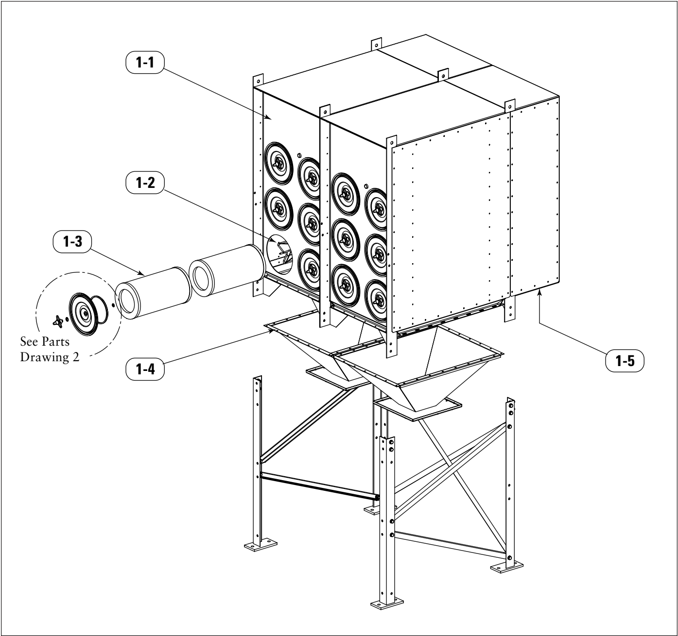
Parts Drawing 1, Downflo II Dust Collector
