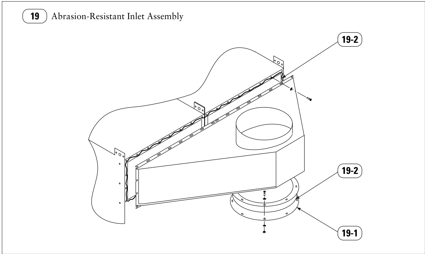
Parts Drawing 19, Abrasion-Resistant Inlet Assembly
